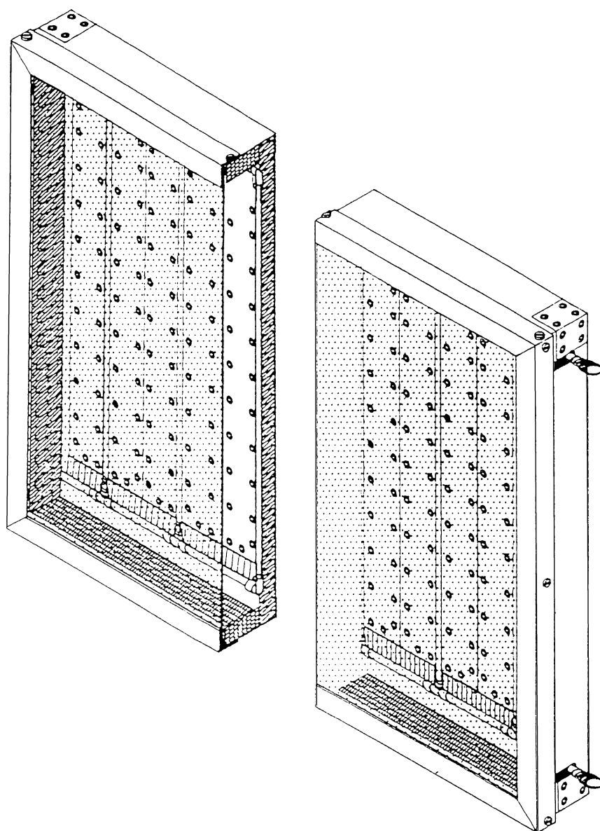
Fig. 1 The solar flat-plate decontaminator with its copper tubes covered by aluminium plates in a box insulated with Rockwool and covered by a double layer polycarbonate plate. The raw water is let in at the bottom, heated and let out at the top through a thermostatic valve
