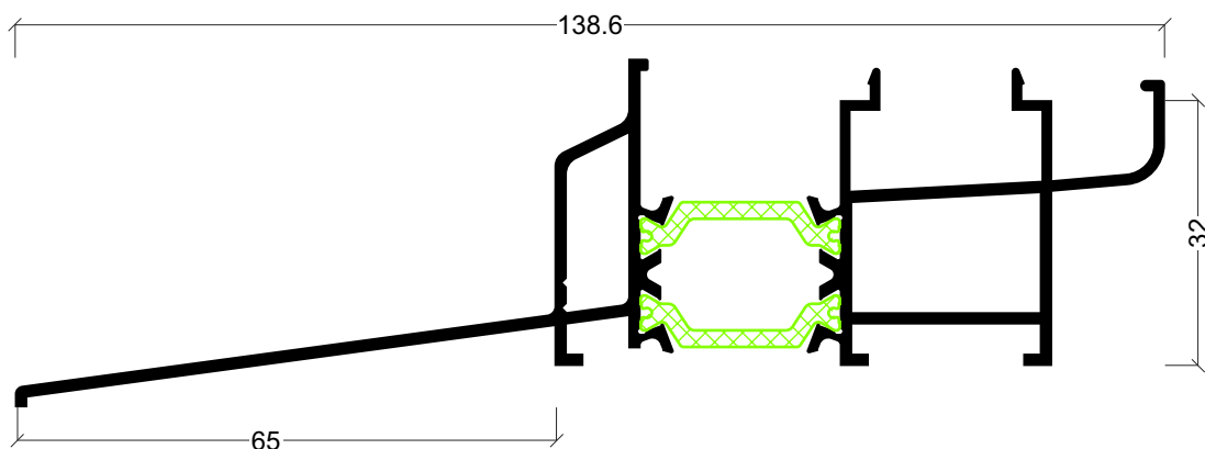
ARi-50 Soleira condensation with drip
