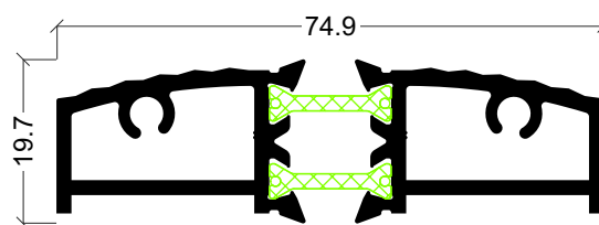
AXi-69 Remate inferior porta
