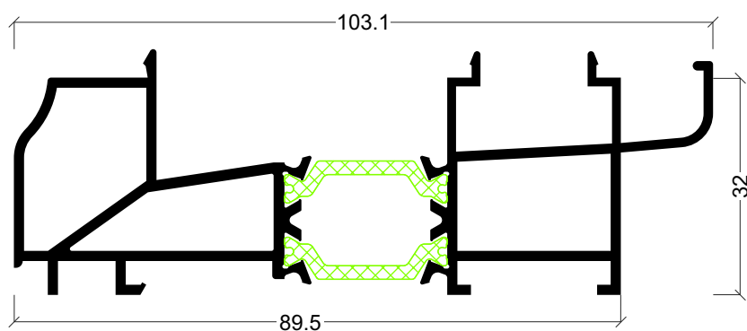
ARi-56 Soleira condensation tradition
