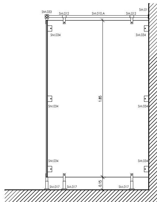
CORTE VERTICAL
